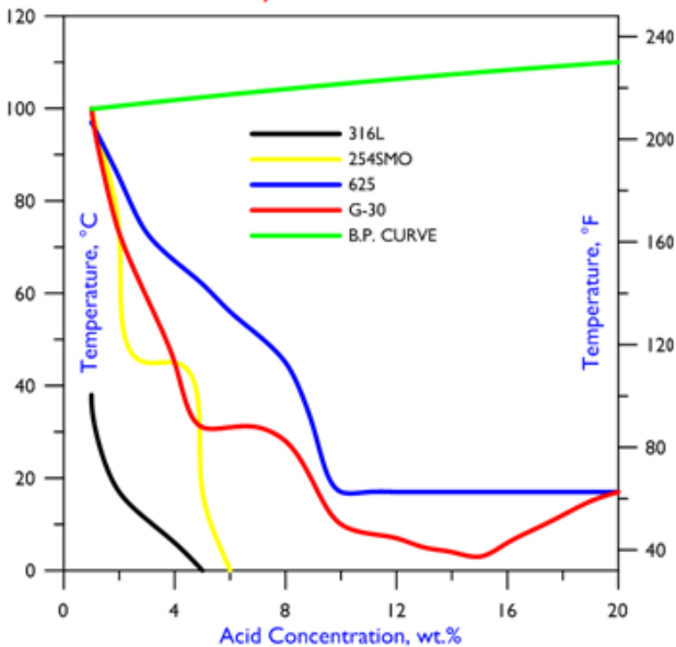
Comparison of 0.1 mm/y Lines in Hydrochloric Acid
